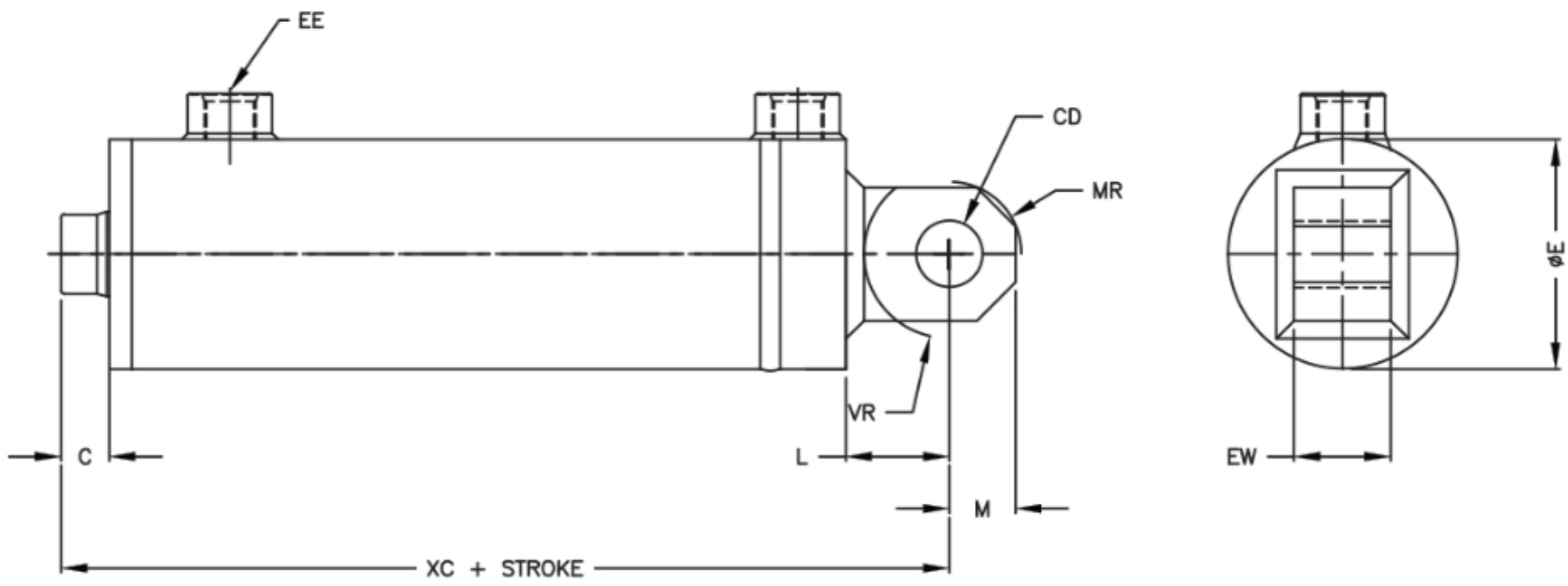
YATES STYLE "V" 1 1/2" - 6" BORE
