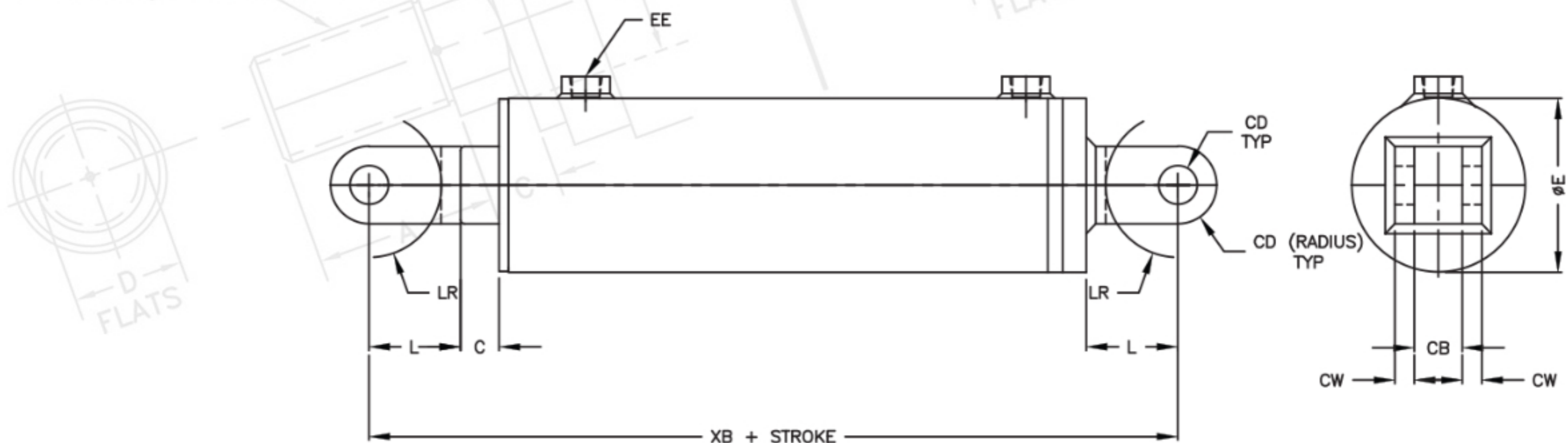
YATES STYLE "B" 1 1/2" - 6" BORE
